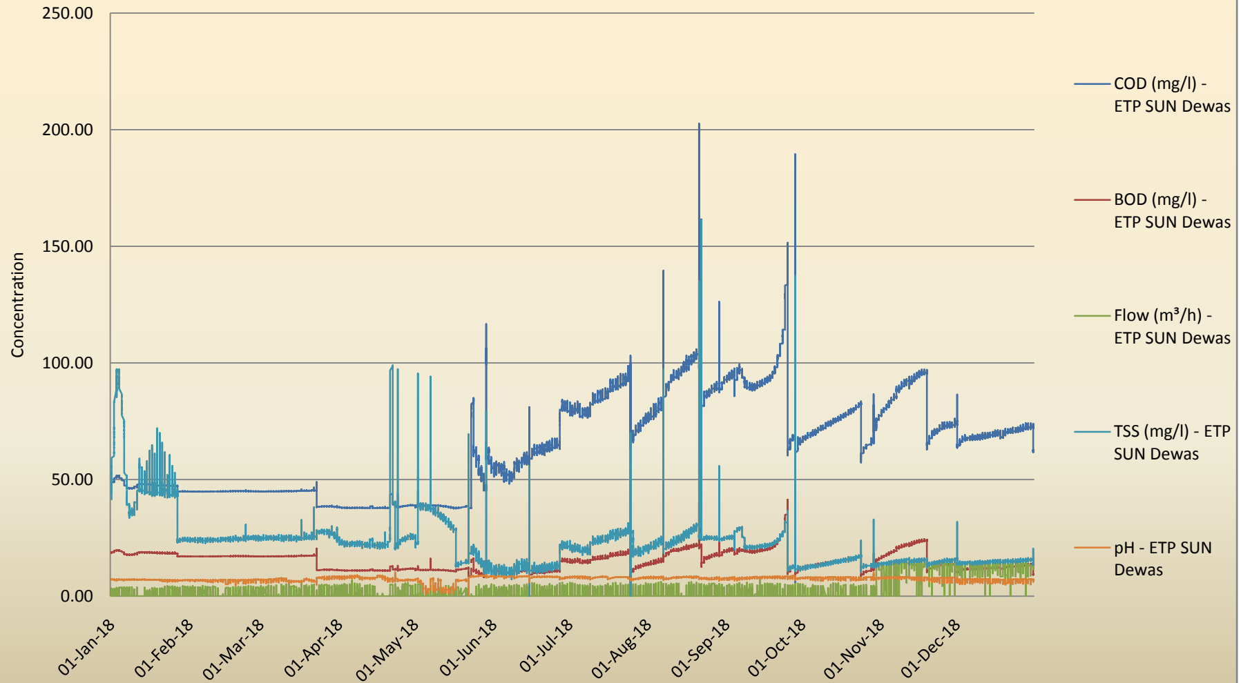
Annual Effluent Trend in M/s. Sun Pharmaceutical Industries Ltd., Dist. Dewas (M.P.)
